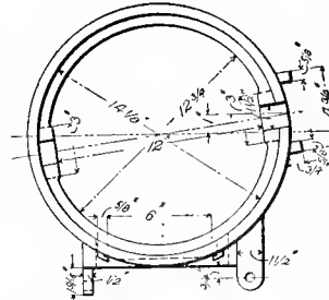
Fig. 3071. Plan of Ash-pit.
